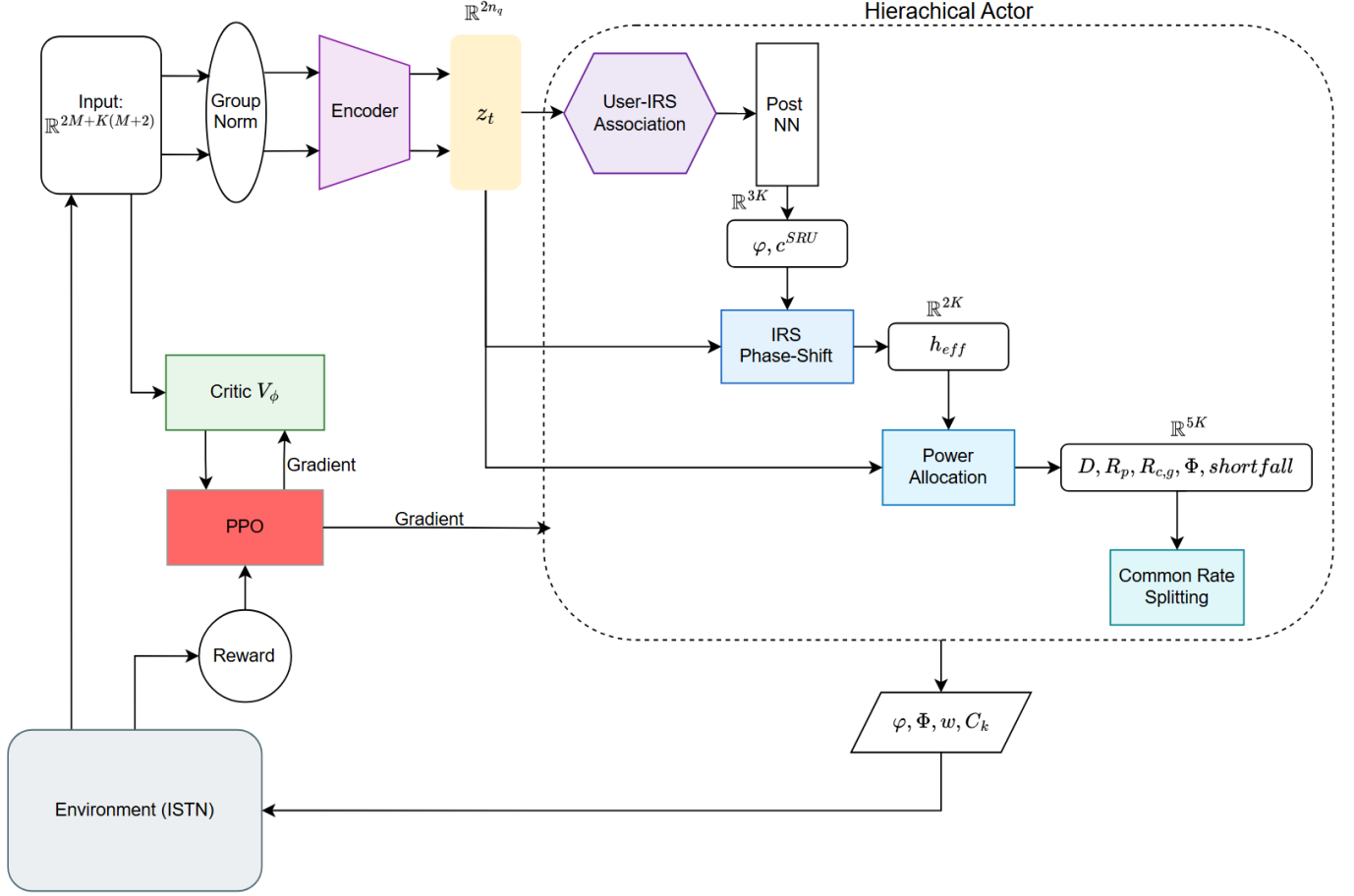
Fig. 2: Overall HQC-HAC hierarchical actor-critic framework. The quantum actor (top level) resolves the discrete IRS-user assignment \varphi via a VQC, while three sequential classical sub-actors (Phase MLP, Power MLP, and Common-Rate MLP) optimize the remaining continuous variables conditioned on the chosen assignment. A shared classical critic provides state-value estimates for computing advantages across all actors.
