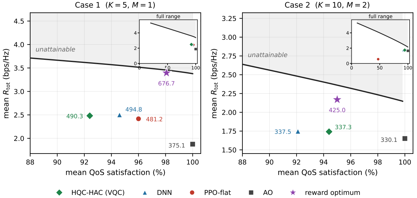
Fig. 7: Rate–QoS frontier and policy operating points for 600 test states per case. The frontier in (29) is obtained by a Lagrangian sweep over the achievable sets; since assignment is exhaustively enumerated and phase is solved exactly, while power splitting is grid-swept, it provides an achievable lower bound, with the shaded region unattainable under this construction. Markers denote the greedy-inference operating points from Table V, annotated by episode return, while stars indicate the reward-optimal operating points over the same achievable sets. The inset shows the full QoS range for Case 2, including PPO-flat.
