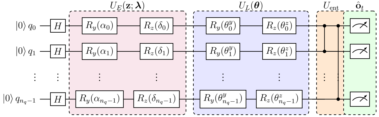
Fig. 4: Variational quantum circuit (VQC) of the quantum actor, shown for representative qubits q_0, q_1, \dots, q_{n_q-1} . Following H^{\otimes n_q} , each layer applies the encoding block U_E(\mathbf{z}; \boldsymbol{\lambda}) , variational block U_L(\boldsymbol{\theta}) , and entangling block U_{\text{ent}} , with data re-uploading across layers. The measurement block marks the readout stage, whose observable set is defined in (19).
